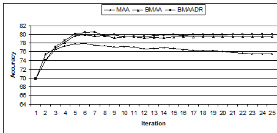
Fig. 1. Accuracies of Merged Algorithms.
